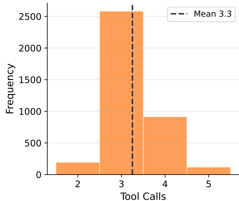
Expected Tool Calls per Record
